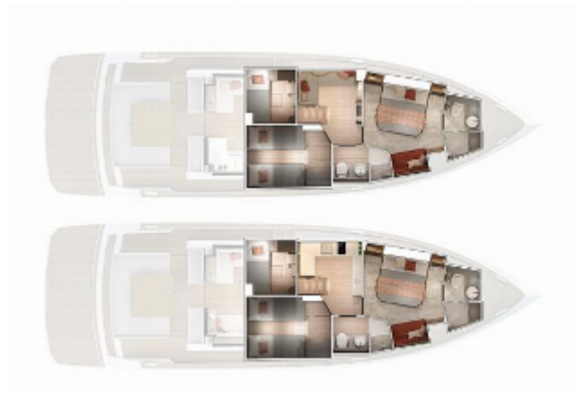
Pardo Yachts GT52 For Sale - Layout
