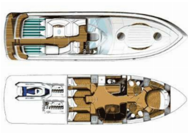
Manufacturer Provided Image: Layout Plan
