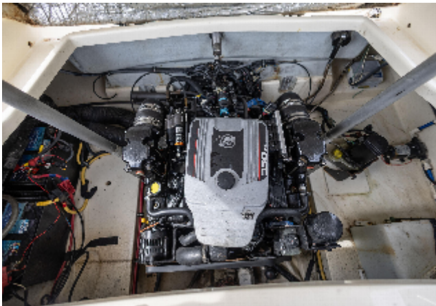
Engine compartment of a 2012 Chris-Craft Launch 25 boat, featuring a 350 MAG engine.
